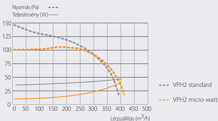
Jelleggörbék
